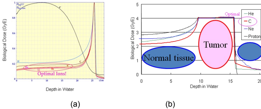
Figure 1. Biological depth-dose distributions of a single Bragg peak with a depth of 26cm (a, presented by A. Brahme in private communication), and 6cm Spread-Out Bragg Peak with a depth of 16cm (b).
