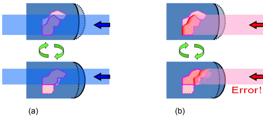
Figure 3. Moving organs due to the respiration. (a) Irradiation by X-rays with the usual external-beam radiotherapy with an electron linac. (b) Irradiation by proton or heavy ions without considerations of the distortion and the density varying.
