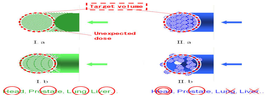
Figure 2. Summary of irradiation methods. I. a Wobbler method. I.b Layer-stacking wobbler method. II.a Pencil-beam scanning method. II.b Pencil-beam scanning method without respiratory gate.
